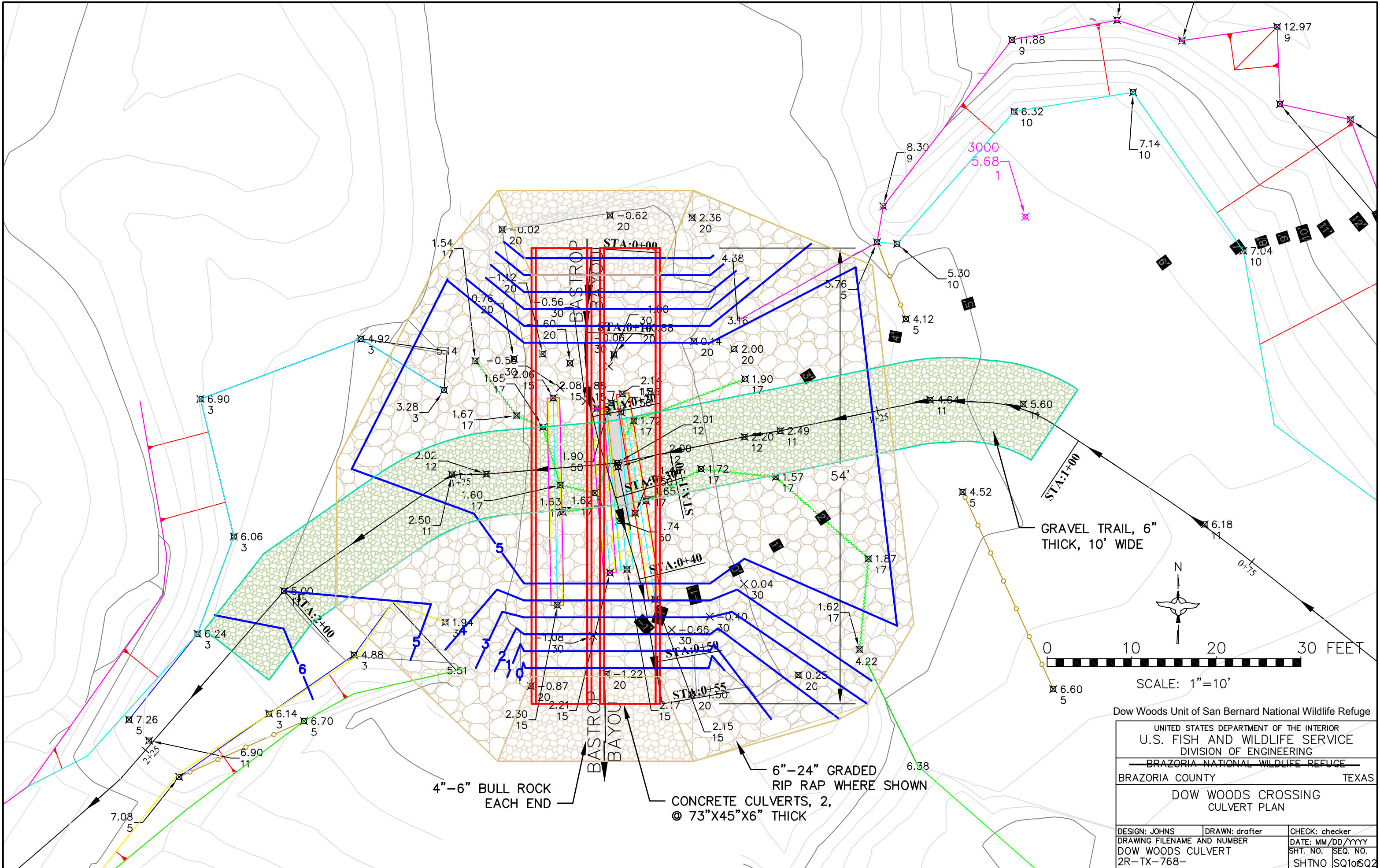
Drawing No. 2R-TX-768-Sheet A
